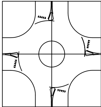
TYP. MARKINGS ROUNDABOUTS W/ONE LANE N.T.S.
