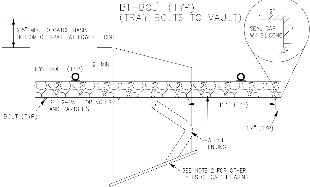
SECTION A-A' PROFILE OF TRAY AND PAVERS TO BE USED WITH TYPE 4-R CATCH BASIN
